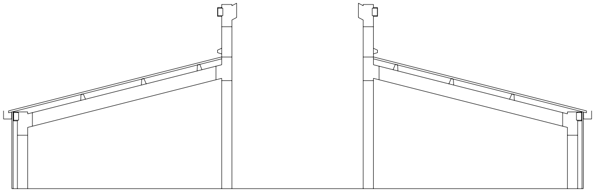
Install Lean-to Roof Sheeting
