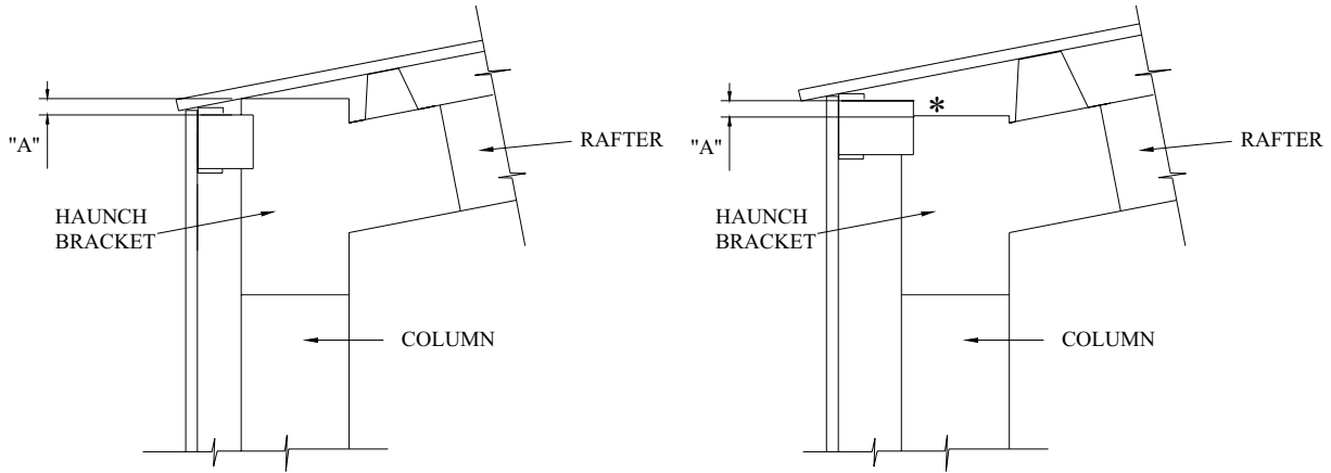
DETAIL - 1
