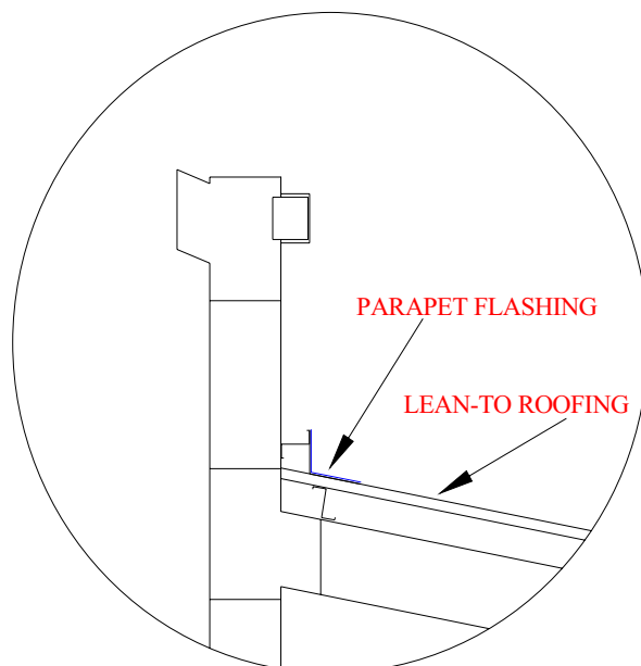
INSTALL PARAPET FLASHING
