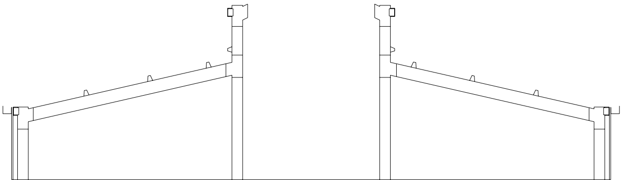
Install Lean-to Roof Purlins
