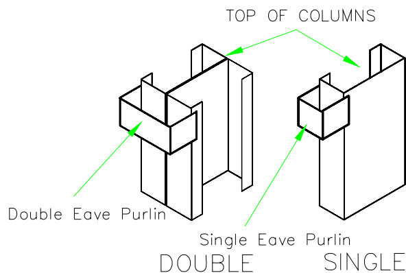
EAVE PURLIN BRACKETS.
