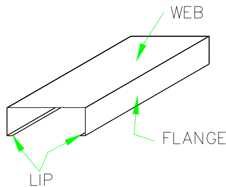
C SECTION.
